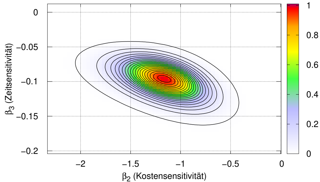
Likelihoodfunktion L(\beta_2, \beta_3, \hat{\beta}_0, \dots)
