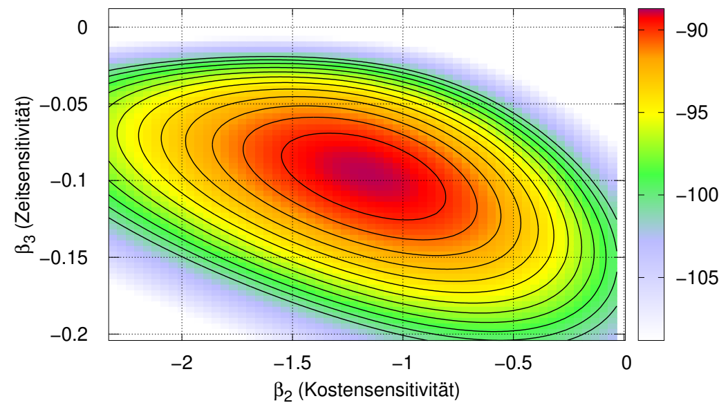
Log-Likelihoodfunktion \tilde{L}(\beta_2, \beta_3, \hat{\beta}_0, \dots)
