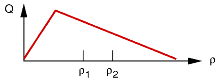
LWR with triangular FD / CTM
